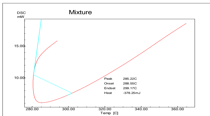
Fig.5: DSC of MESALAMINE +Guargum+Xanthan gum+ Acacia gum
