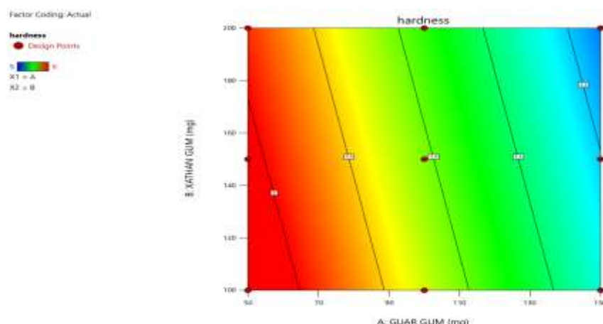
Fig. 11: Contour plot and Response surface plot showing the effect of concentration of Guar gum(x1) and Xanthan (x2) on hardness (y2)
