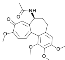
Fig. 1: Colchicine
