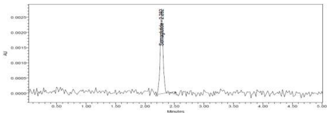
Fig 3: LOD Chromatogram of Semaglutide
