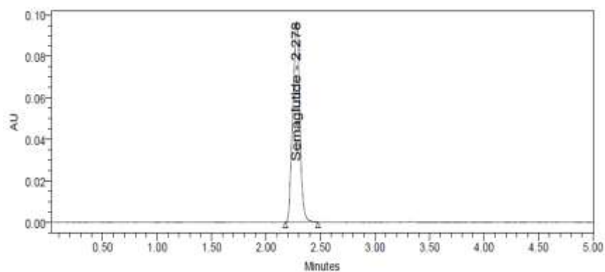
Fig 5: Assay Chromatogram
