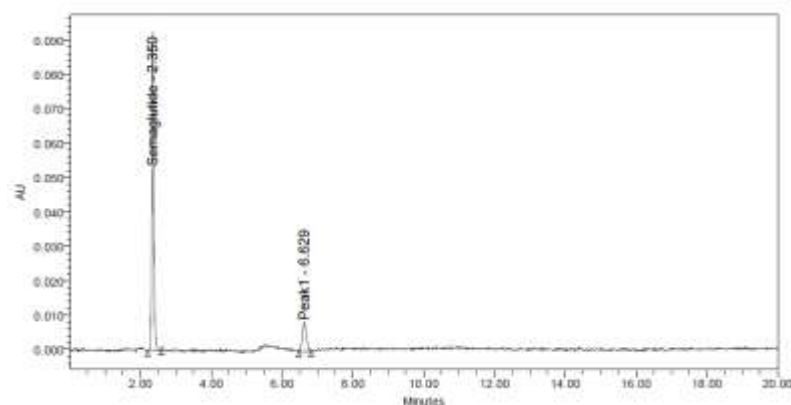
Fig 10: UV degradation chromatogram
