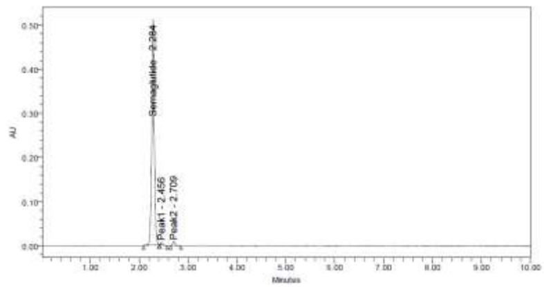
Fig 8: Peroxide degradation chromatogram
