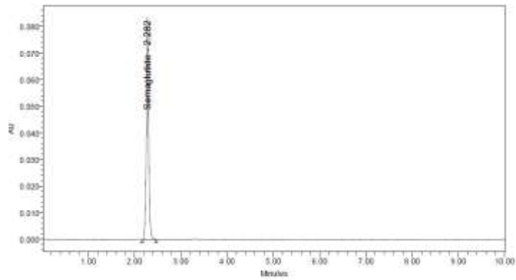
Fig 9: Thermal degradation chromatogram
