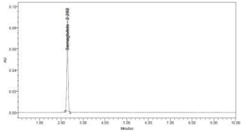
Fig 7: Base degradation chromatogram
