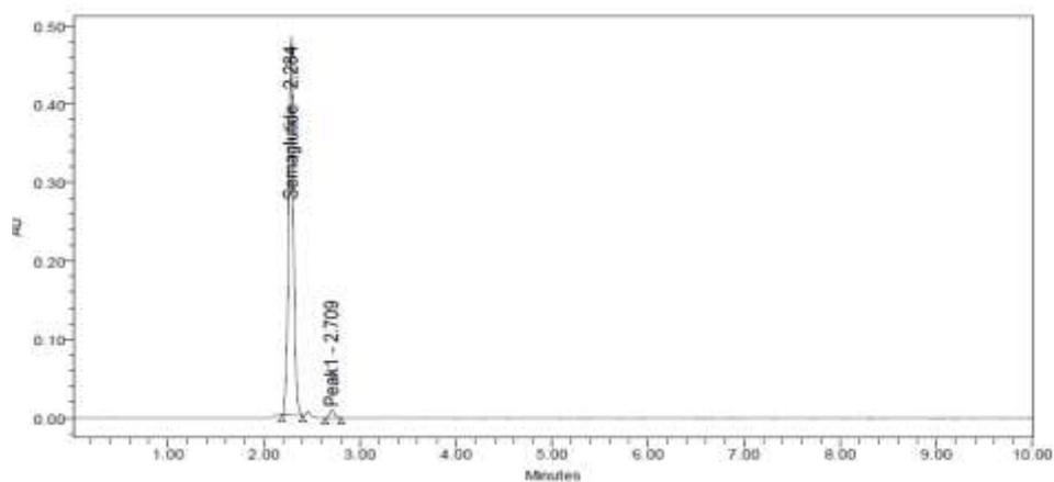
Fig 6: Acid degradation chromatogram
