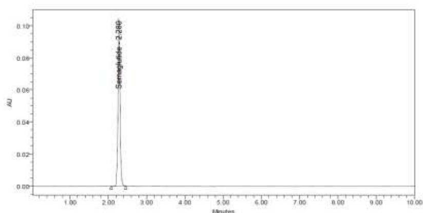
Fig 11: Water degradation chromatogram
