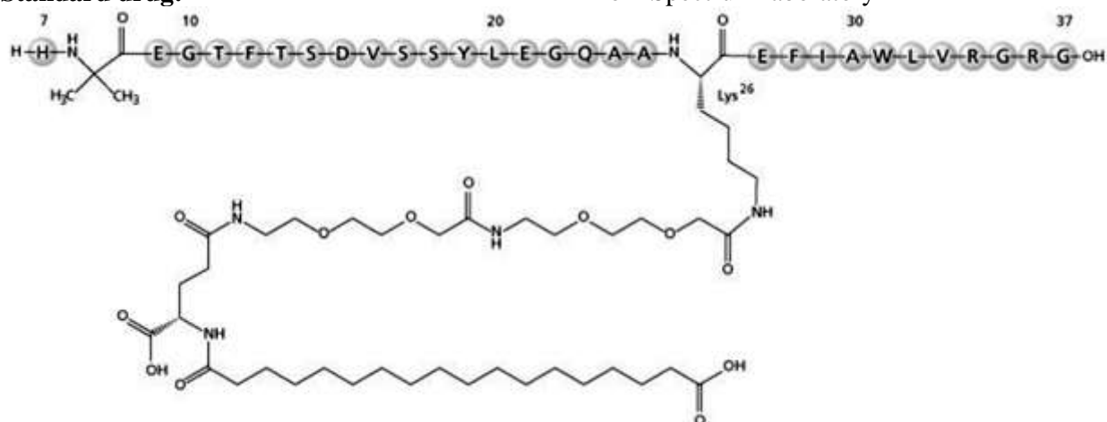
Fig: 1 Chemical Structure of Semaglutide
